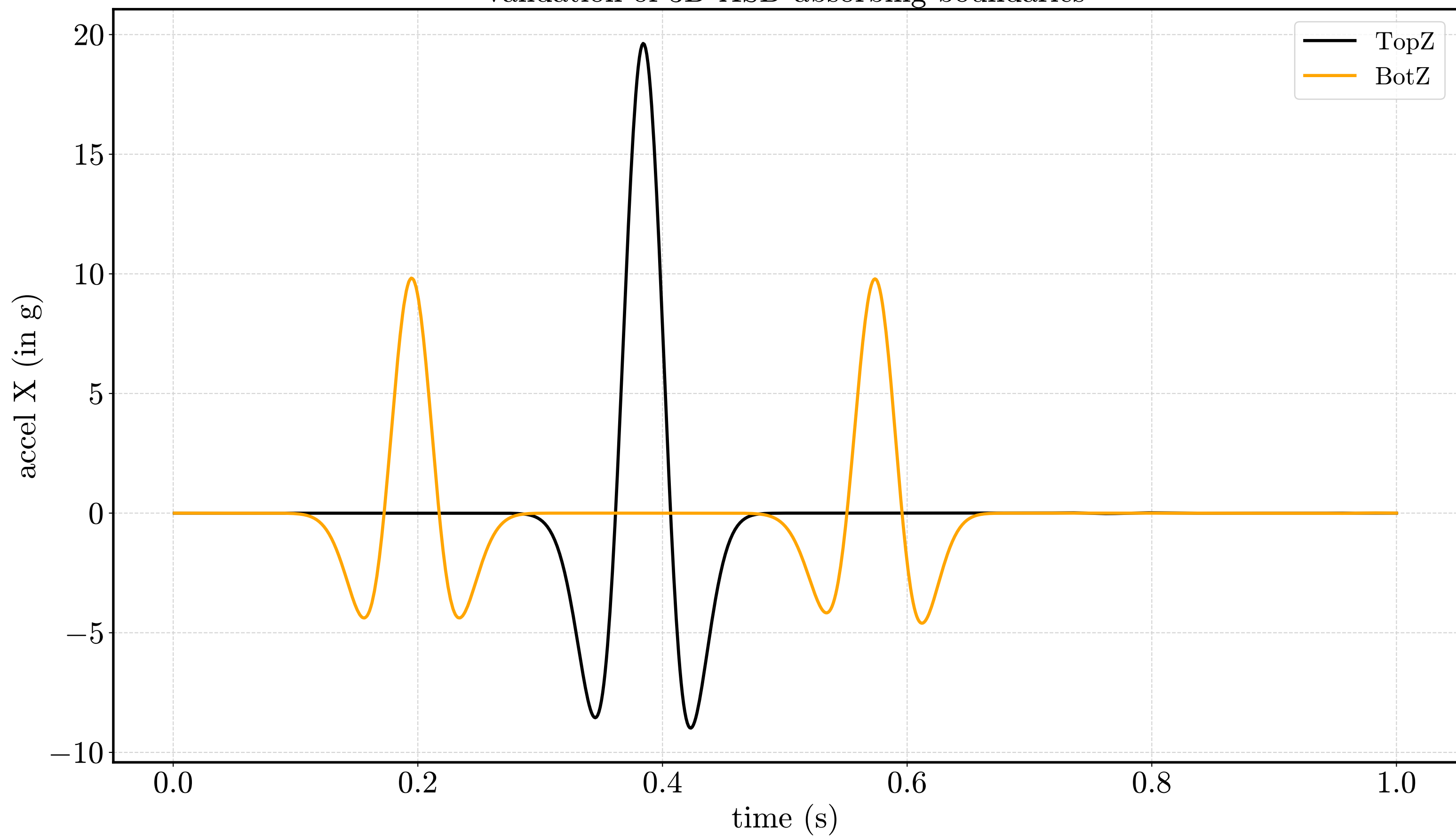
validation of 3D ASD absorbing boundaries
